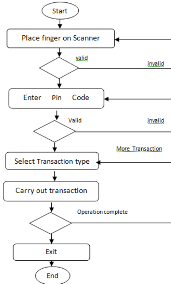
Fig-4: Authentication Phase
